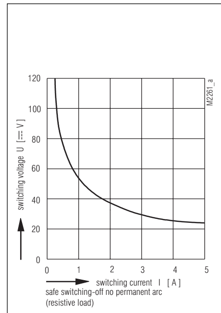
Limit curve for arc-free operation (at t_u = 20^\circ\text{C} ) for OW 5691 and OW 5699 safe switching-off no permanent arc (resistive load)
