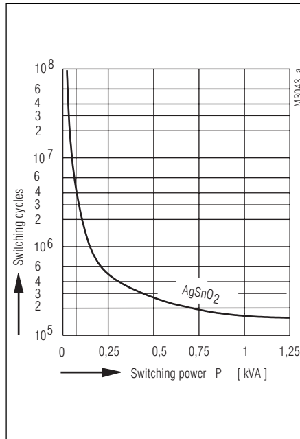
Contact service life for OW 5691 and OW 5699 with I_{th} \leq 5 A (NO contact)
