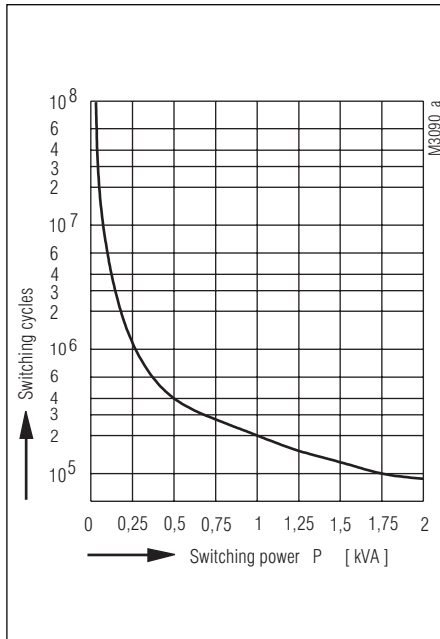
Contact service life for OW 5699 with I_{th} \leq 8 A (NO contact)
