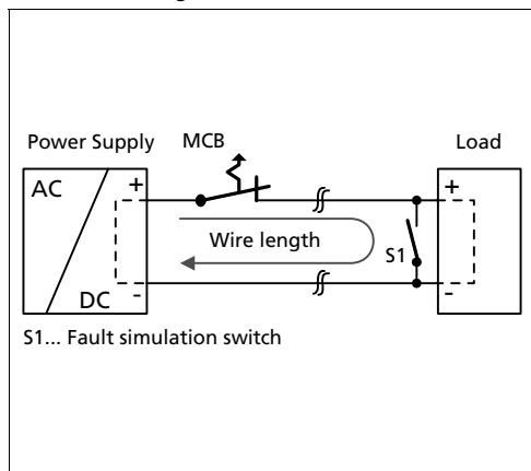
Fig. 24-5 Test circuit
